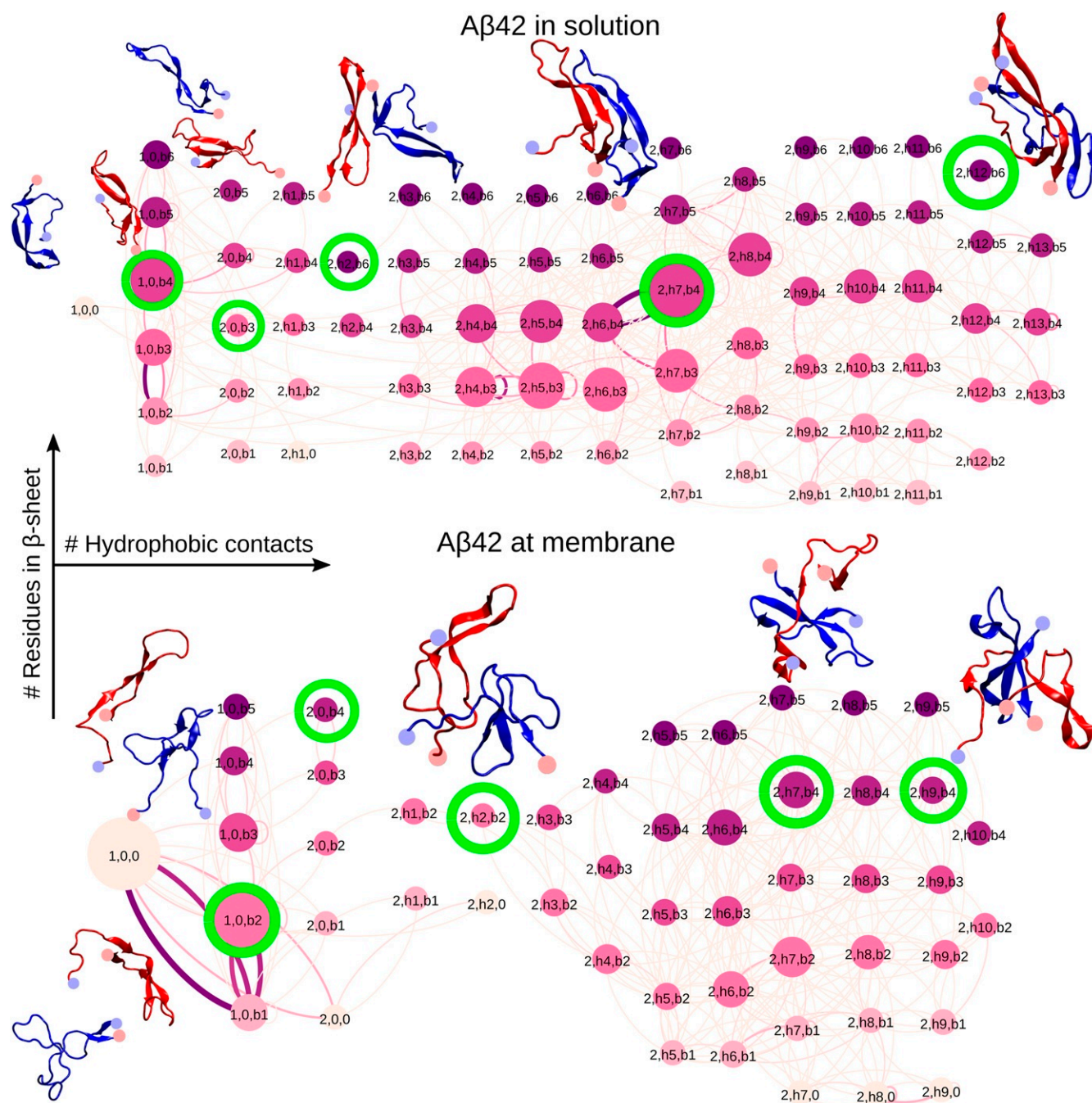
Fig. 4. The TN for A \beta 42 dimerization in the aqueous phase ( Top ) and in the presence of the neuronal membrane ( Bottom ). Each node is defined by three descriptors: oligomer size, number of interpeptide hydrophobic contacts, and number of residues in \beta -strand conformation. The last two descriptors are grouped in blocks of five and are named h1 to h12 for hydrophobic contacts and b1 to b6 for the number of residues in \beta -strand conformation. The nodes are connected by edges that represent transitions between the connected peptide states. The size of the nodes and the thickness of the edges are proportional to the respective state or transition probability. They are colored based on the descriptor reflecting the number of residues in \beta -strand conformation (from light pink for no \beta -sheets to dark purple for the maximum amount of \beta -sheets in b6). For the nodes circled in green representative peptide conformations are shown (see color code in Fig. 2).
